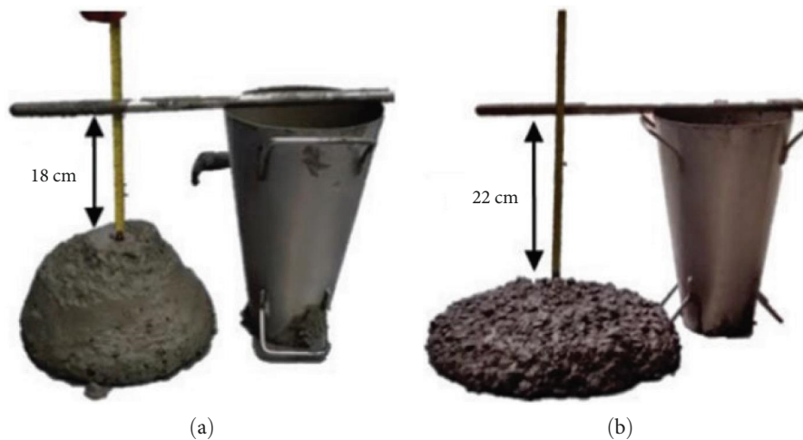
FIGURE 1: Slump test of concrete mixture (a) only by OPC and (b) OPC + alkali activated by natural pozzolana from Robayo-Salazar et al. [58].
